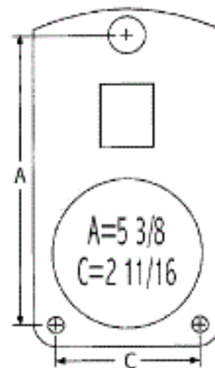
Axle Hole Spacing
